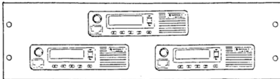
ACP2605C THREE MCS2000 MODEL ONE IN A 5 1/4"H X 19"W PANEL
