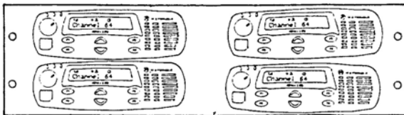
ACP 2623D FOUR CDM1250 IN 5½"H X 19"W PANEL.
