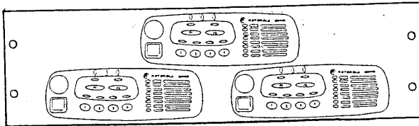
ACP2621C THREE CDM750 RADIOS IN 5 1/4"H X 19"W PANEL.
