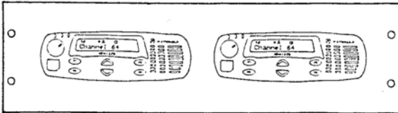
ACP 2623B TWO CDM1250 IN 5½"H X 19"W PANEL.
