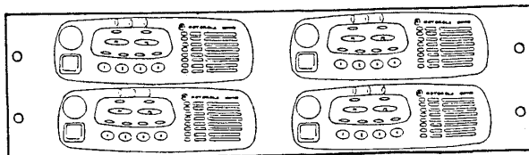
ACP2621D FOUR CDM750 RADIOS IN 5 1/4"H X 19"W PANEL.
