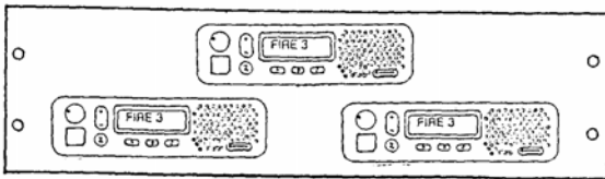
ACP 2622C THREE CDM1225 IN 5 1/4" X 19"W PANEL.
