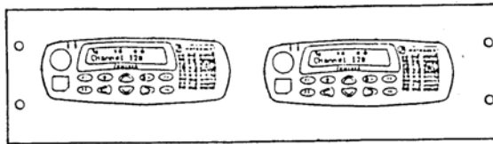
ACP 2624B TWO CDM1550 IN 5 1/4" H X 19" W PANEL.
