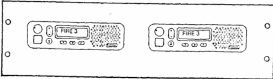
ACP 2622B TWO CDM1225 IN 5 1/4"H X 19"W PANEL.
