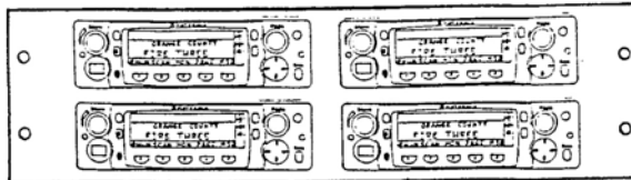
ACP 2631F FOUR XTL5000 IN 5¼"H X 19"W PANEL. (NO SPEAKERS)
