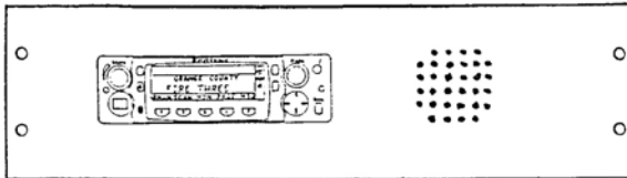
ACP 2631A XTL5000 IN 5¼"H X 19"W PANEL WITH SPEAKER. (SPEAKER PROVIDED)
